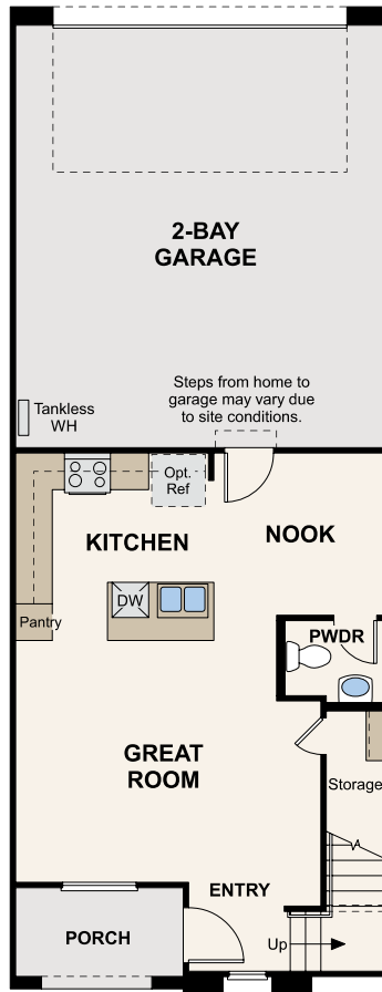
MAIN LEVEL
